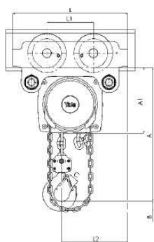
Yalelift ITP, 500 - 3.000 kg
