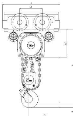
Yalelift ITP/ITG, 5.000 kg
